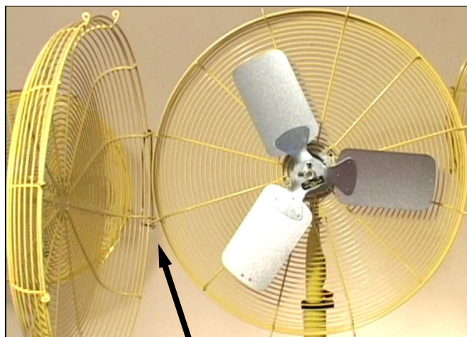
Hinging Guard Safety Hinge Pin (J)
