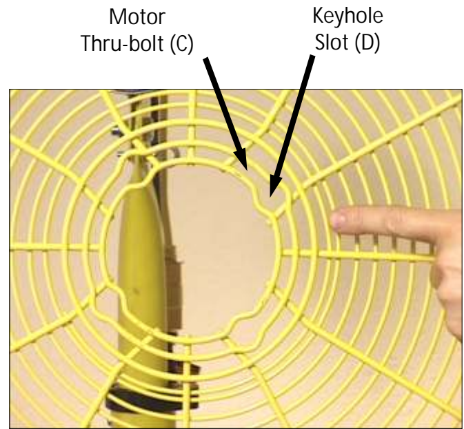
Quick Mounting Ring
